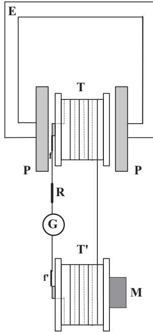
Figure 1: experimental setup used by Blondel. See text.
